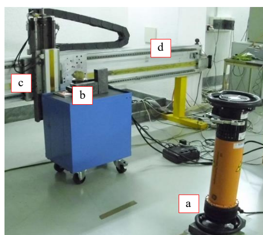
Figure 2. The tomographic set-up used for the analysis (a: source; b: sample; c: detector; d: movement system)
