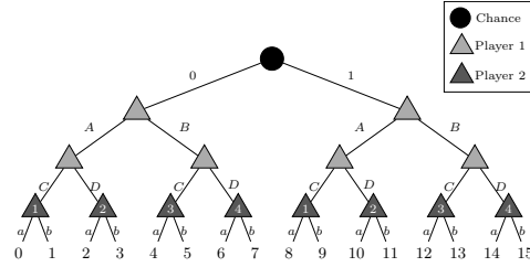
Figure 3: Extensive form of a 2-player team game with chance and without adversary, where Player 2 observes all actions except those of chance. Nodes of a player with same number are in the same info set.
