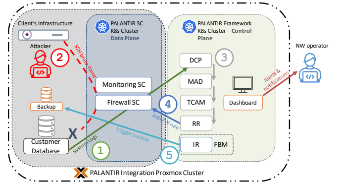
Fig. 3. Workflow for storyline #2
