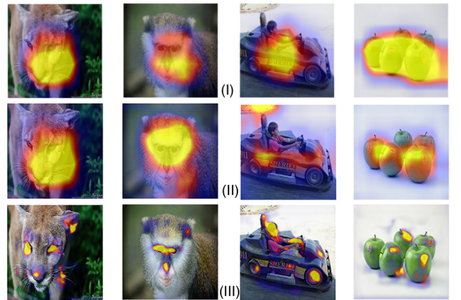
Fig. 2. GradCAM++ explanation maps: (I) ResNet50, (II) VGG16, (III) U-Net.
