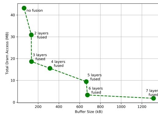
Figure 13. Minimum storage to fuse VGG16 layers.
