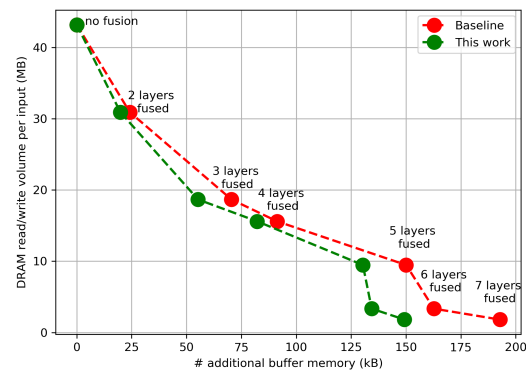
Figure 12. Reuse buffer comparison against [12].
