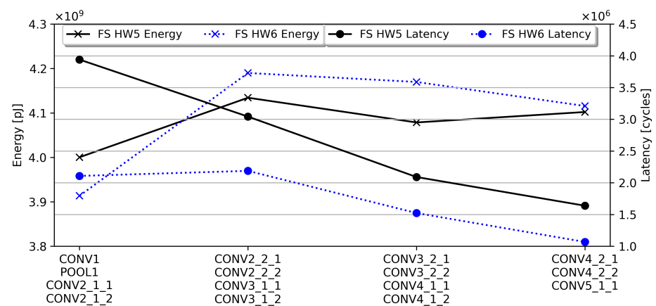
Figure 17. Energy and latency for VGG16, mapped with temporal fusion with HW config. 5 and 6.
