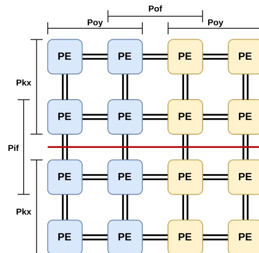
Figure 3. Example of row-stationary mapping.
