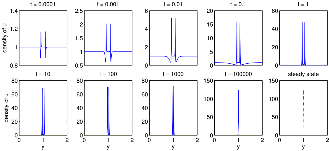
Figure 4: Simulation showing the time evolution of solutions to equation (6.3) with u_0(y) = 1 and d_2(y) as in (6.1) with \varepsilon = 0.01, a = 0.9 and b = 1.1 . The population initially accumulates into two concentrated peaks at y = a and y = b , which subsequently undergo slow convergence to a single peak in the centre of domain. The final panel plots the analytically determined steady state solution. Simulations performed as described in the text, where we have again employed a variable mesh. Error tolerances as in Figure 3.
