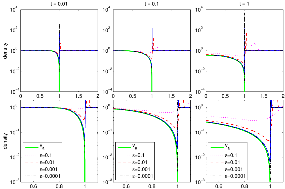
Figure 6: Comparison between solutions to the 1D diffusion model (6.3) and the analytical solution (6.6) to the Dirichlet problem. For (6.3) we consider u_0(y) = 1 , d_2(y) as in (6.1) for varying \varepsilon and a = 1 . The top row plots the \log_{10} of the population density against y for various values of \varepsilon at the times indicated. In each frame we add the analytical solution v_a(y, t) for the region y \in [0, a) . The bottom row expands the bottom-left corner of these plots to reveal the convergence to the analytical form. Simulation method as described in Figure 4.
