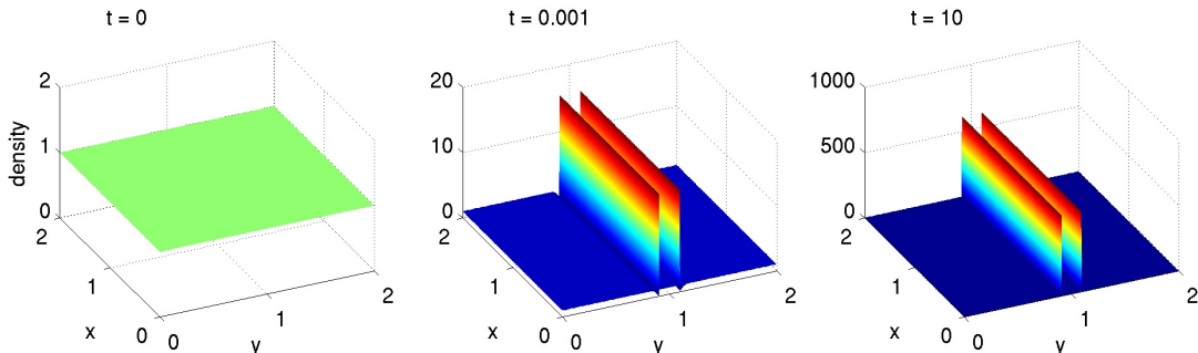
Figure 2: Simulation of the anisotropic diffusion model, system (1.4) together with u_0(x, y) = 1 and smooth diffusion coefficients given in (6.1). Time evolution showing solutions using \epsilon = 0.001 , a = 0.9 and b = 1.1 . The population accumulates into two extremely concentrated ridges at the interface between the isotropic and aligned regions, with negligible subsequent movement within simulation timescales. Simulations performed as described in Section 6.
