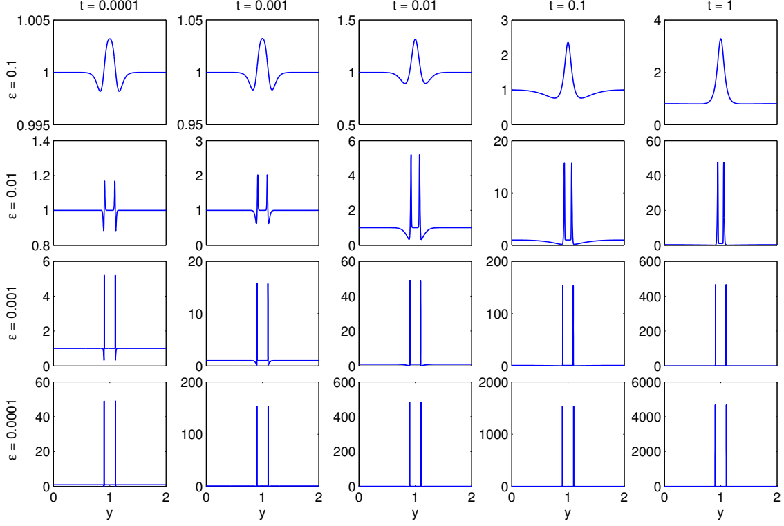
Figure 5: Simulation of the 1D diffusion model, equation (6.3), together with u_0(y) = 1 and d_2(y) as in (6.1) for varying \varepsilon , a = 0.9 and b = 1.1 . In the top to bottom rows we compare the evolution of solutions at comparable times for \varepsilon = 0.1, 0.01, 0.001 and 0.0001 . As \varepsilon \rightarrow 0 we note that solutions become more sharply concentrated into aggregates at y = a and y = b . Simulation method as described in Figure 4.
