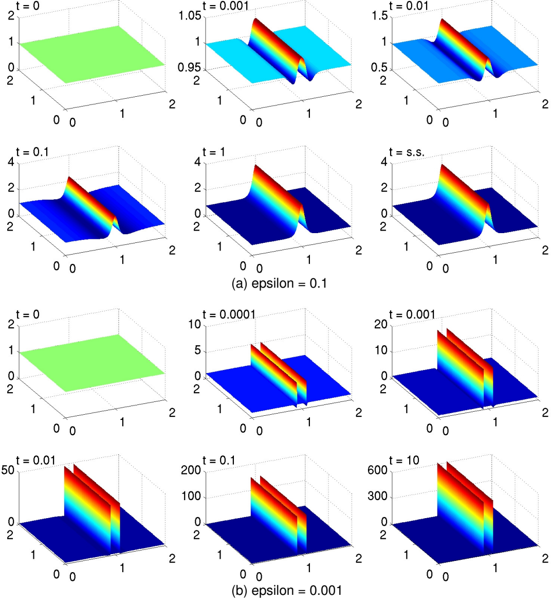
Figure 3: Simulation of the anisotropic diffusion model, system (1.4) together with u_0(x, y) = 1 and the smooth form (6.1). (a) Time evolution showing solutions using \epsilon = 0.1 , a = 0.9 and b = 1.1 in (6.1). The population accumulates inside the aligned region, evolving to a heterogeneous steady state distribution. The analytically-determined solution steady state solution is shown in the final panel. (b) Time evolution showing solutions using \epsilon = 0.001 , a = 0.9 and b = 1.1 in (6.1). The population accumulates into two extremely concentrated ridges at the interface between the isotropic and aligned regions, with little subsequent movement within simulation timescales. Simulations performed as described in the text. Here we have employed a variable 2D mesh, concentrating points at the aligned region to provide better resolution of the ridge development. Absolute and relative tolerances for the time-integration scheme were set at 10^{-8} .
