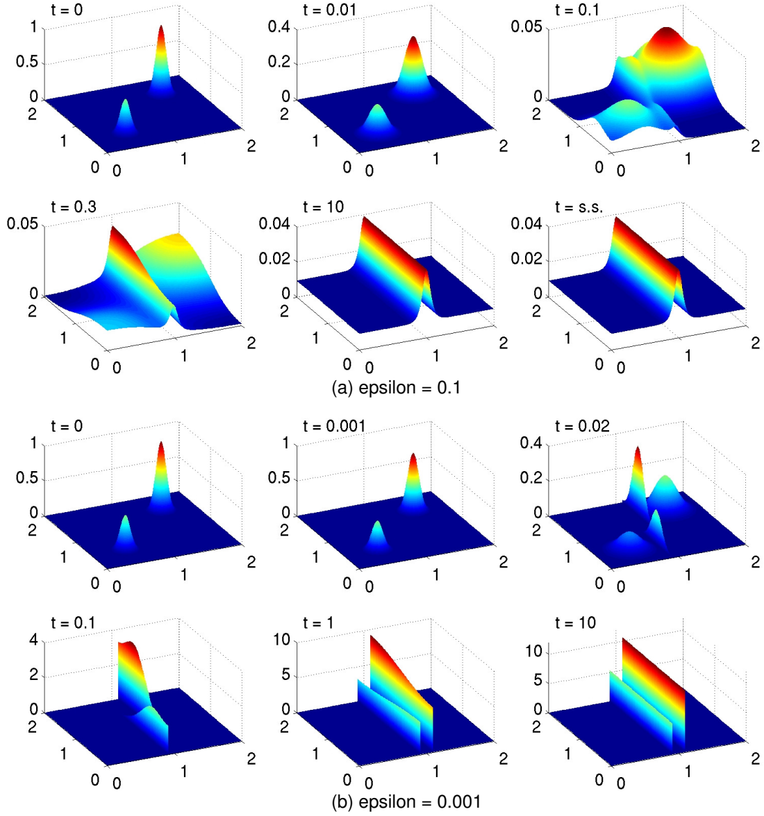
Figure 7: Simulation of the anisotropic diffusion model, system (1.4) with nonuniform initial conditions (see text for details). (a) We set \epsilon = 0.1 , a = 0.9 and b = 1.1 in (6.1). (b) We set \epsilon = 0.001 , a = 0.9 and b = 1.1 in (6.1). For details of numerical implementation, see Figure 3.
