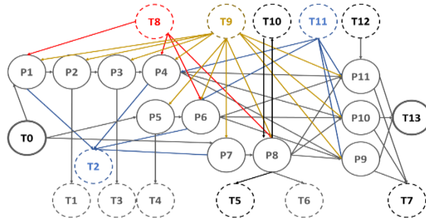
e) The complete RA MEIO graph.
