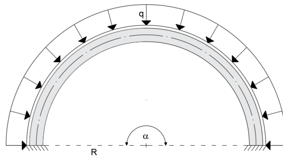
Fig. 5. Uniform circular beam under uniformly distributed load.
