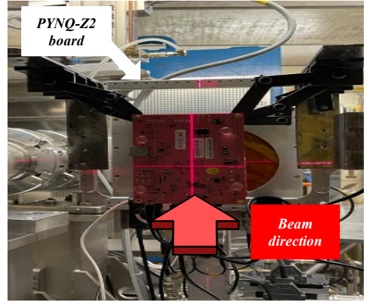
Fig. 6. Board exposed to the protons beam.
