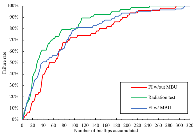
Fig. 11. Failure rate with the accumulation of fault injections and radiation test data.
