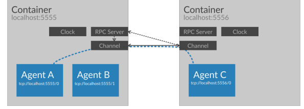
Fig. 2: Agents-Containers architecture [15]
