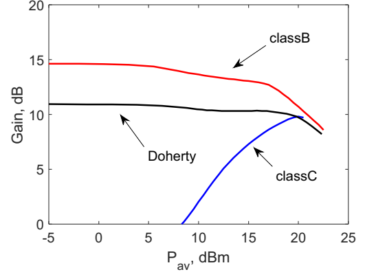
Figure 9: Gain of the DPA compared to parallel class B and class C stages. The same P_{av} has been fed to each stage for comparison.
