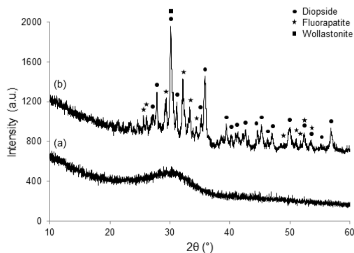
Figure 3. XRD plot of (a) 1d glass and (b) 1d glass-derived scaffolds (ground into a powder) produced by sintering at 800^\circ\text{C} for 3 h.
