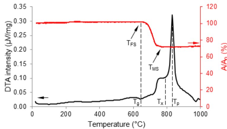
Figure 2. Thermal analyses of 1d glass: DTA and HSM.
