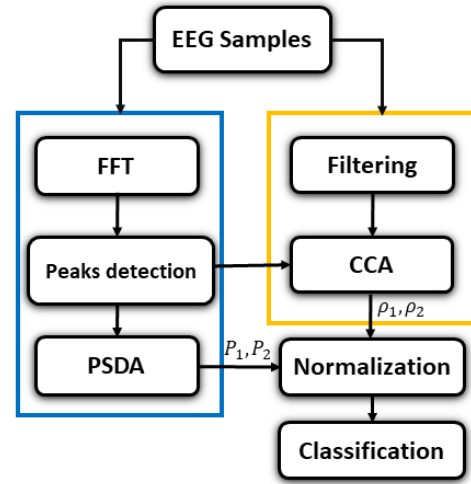
Fig. 4. SSVEP Classification Algorithm with processing in frequency (blue box) and time (yellow box) domain.
