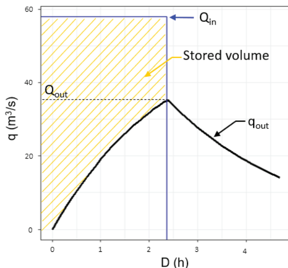
Figure 2. Example of flood attenuation for the Agaro dam (Piedmont region, A_B = 11 \text{ km}^2 , A_L = 0.06 \text{ km}^2 , W = 36\text{m} ).
