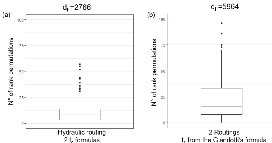
Figure 3. Boxplots of the distribution of rank permutations for each dam. Panel (a) refers to different formulations for the time of concentration within the complete method, panel (b) refers to the difference between the two methods, for the same time of concentration (i.e. the one by Giandotti).
