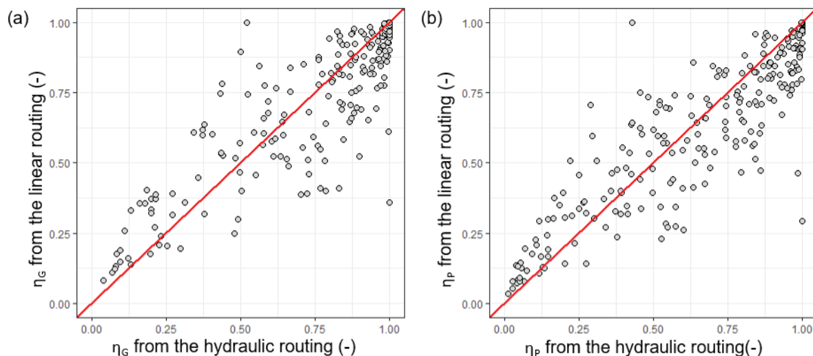
Figure 5. Results from the linear routing compared with those from the integration of the differential equation of the lakes, for the Giandotti's (a) and the Picking's (b) time of concentration.
