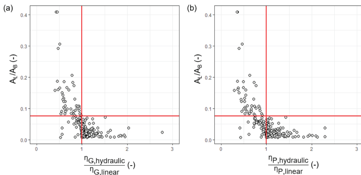
Figure 6. Ratio between the attenuation coefficients obtained with the two routing methods with the Giandotti's (a) and the Picking's (b) time of concentration.
