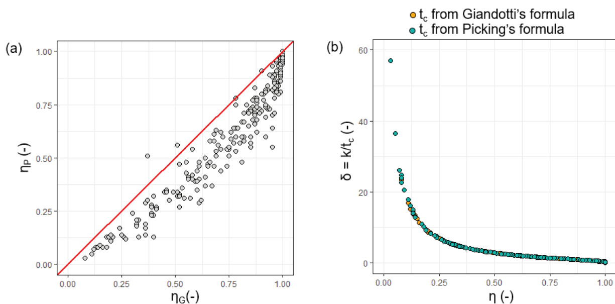
Figure 4. (a) Comparison between the \eta values computed with different formulation for the time of concentration. (b) Analytical relationship linking \eta to the \delta parameter.
