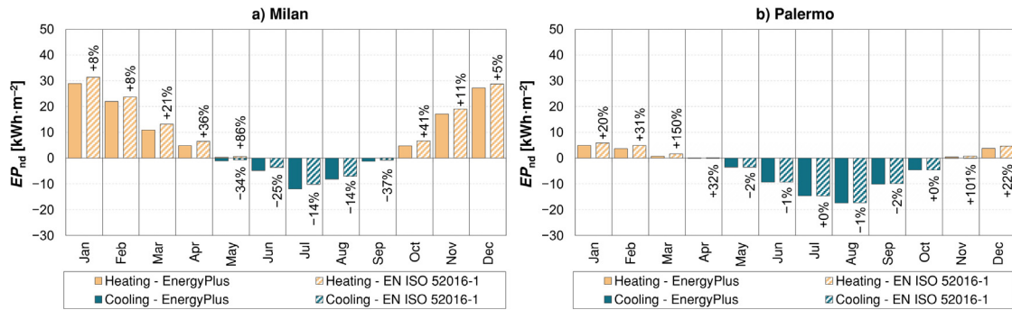
Fig. 5. Monthly thermal energy needs of the building from the standard and the full detailed model for Milan (a) and Palermo (b).
