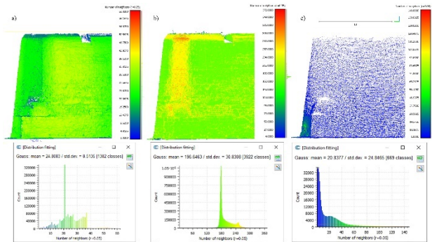
Figure 8. Density analysis (radius 5 cm). left) optimized Lidar data; middle) close-range photogr. data; right) SLAM data.
