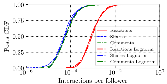
Fig. 28 CDF of the total number of interactions per follower (measured as reactions, shares, and comments per follower) on influencer Laura Pausini (singer) on FB at the end of the posts’ lifetime, along with their log-normal fit
