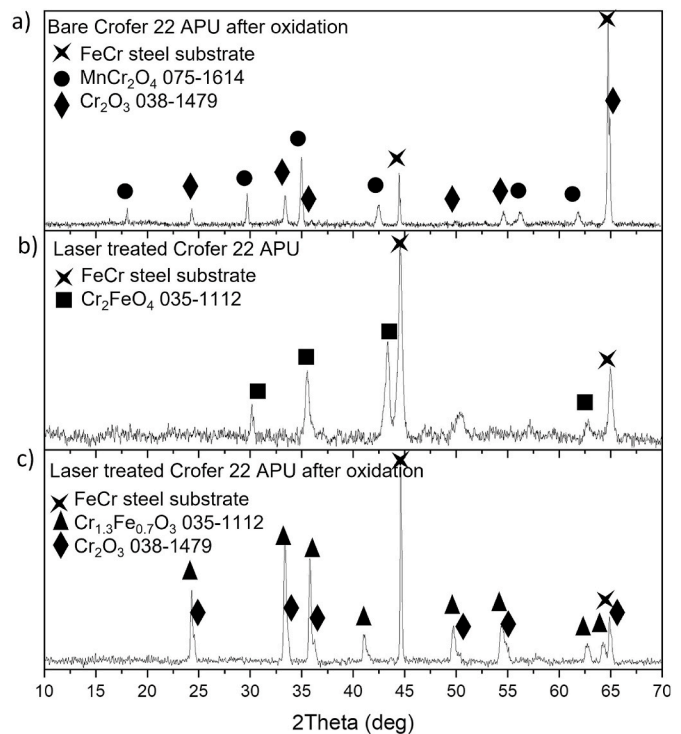
Fig. 3. XRD patterns of bare Crofer after oxidation (a) laser-processed Crofer(b) and laser-processed Crofer after oxidation treatment (c).
