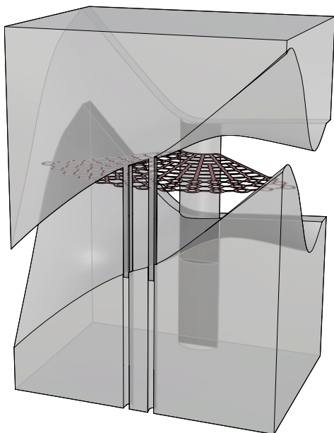
Fig. 3. Modelled dies and undeformed MatrixMIDFACE orbital plate.
