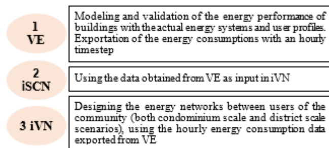
Figure 7. Software workflow
