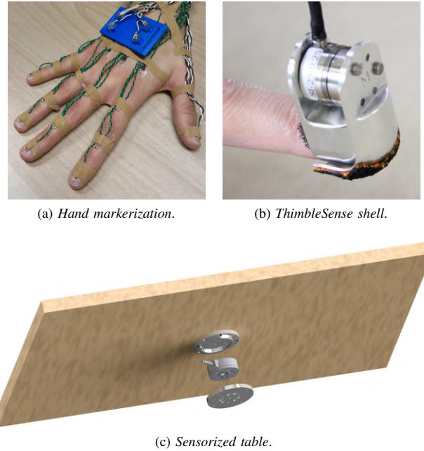
Fig. 2. a) 24 markers are fastened to hand and phalanges for hand kinematic tracking. b) The tactile impairment is obtained by wearing ThimbleSense shells on fingertips. c) Exploded view of the sensorized platform used in the experiments.
