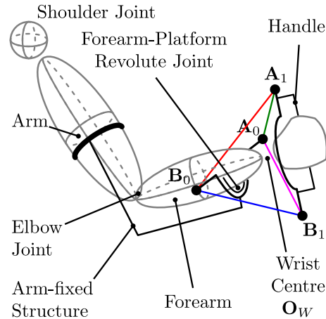
Fig.2b Diagram of the robot working principle. The patient joints are not represented for more clearness. Cable P_1 is green, P_2 is red, P_3 is magenta, and P_4 is blue
