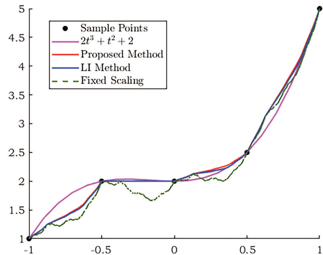
FIG. 2. Approximation of 2t^3 + t^2 + 2 using three various scaling factors I_j , I_j^* , and I_j^{**} .
