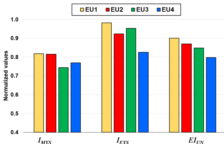
Figure 2. Case Study A. United Nations Education Index, EI_{UN} , and its components: I_{MYS} (normalized Mean Years of Schooling), I_{EYS} (normalized Expected Years of Schooling). This data are referred to the last year available for the OECD PISA assessment (2018). Raw data of the UNs indicators are available in Refs [56–58].
