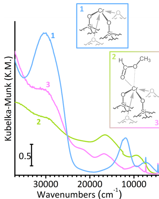
Figure 6. DR UV-Vis spectra of three Cr(II)/SiO 2 catalysts obtained from Cr(VI)/SiO 2 by different reduction treatments: in CO at 350 °C (spectrum 1), in ethylene at 150 °C (spectrum 2) or in ethylene at room temperature under UV irradiation (spectrum 3). In the latter two cases, the spectra are collected when the majority of Cr(VI) sites have been reduced but before the onset of the ethylene polymerization reaction. The differences with respect to spectrum 1 are due to the presence of the by-products of ethylene oxidation in the Cr(II) coordination sphere, as schematically depicted in the sketches.
