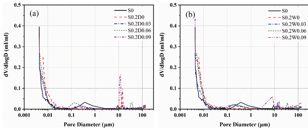
Fig. 11. Pore size distribution of AAS mortar with SAP with different liquid-binder ratios: (a) Dry mixing, (b) Wet mixing.
