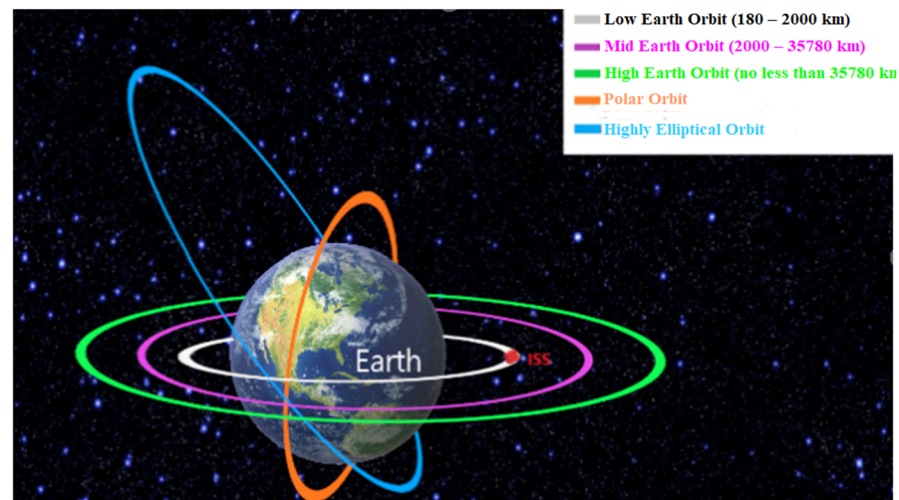
Figure 2. Altitude classifications for geocentric orbits.
