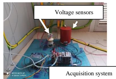
Figure 2. Measurement setup arranged in the DC substation. Scheme a) and picture a) of the setup.
