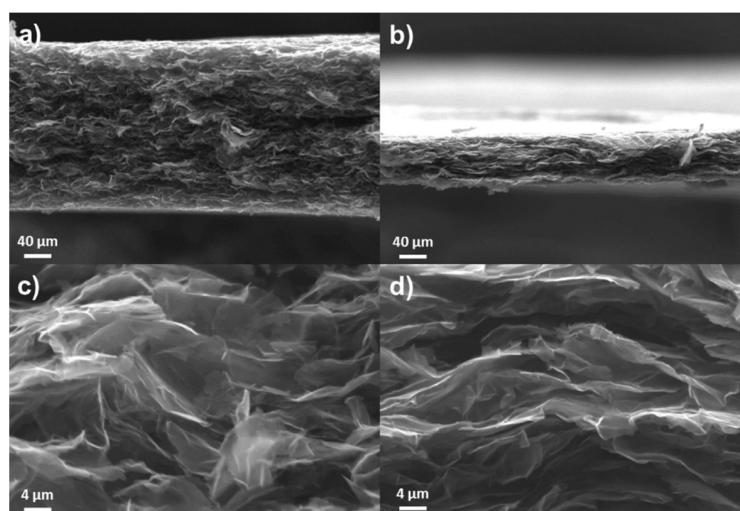
Figure 1. SEM micrographs of pristine GNP nanopaper: unpresseed (a,c) and pressed (b,d). Dark areas in between flakes correspond to porosity of the nanopapers.
