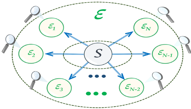
FIG. 2. Quantum Darwinism recognizes that information about a system S is obtained from disjoint environment fragments consisting of distinct subsystems \varepsilon_i 's of \mathcal{E} by independent observers. Unconstrained proliferation of classical correlations means that only the information about a pointer observable is accessible. Equation (7) implies that, whenever classical objectivity manifests, bipartite quantum correlations are suppressed.
