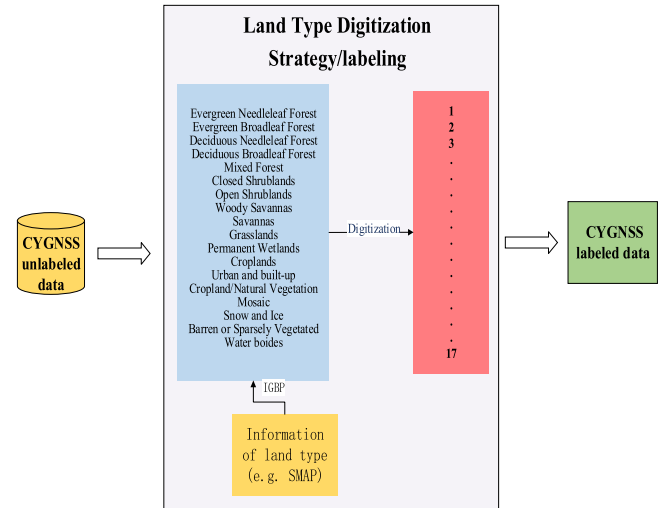
Fig. 5. Proposed LT digitization strategy that integrates land surface information.
