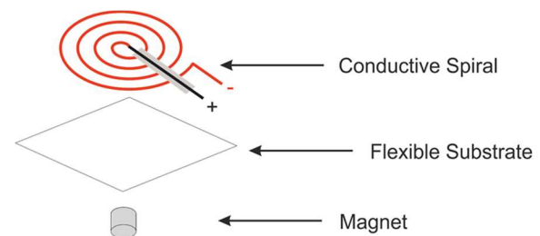
Figure 1: Schematic of the electrodynamic planar loudspeaker with a conductive spiral, a flexible substrate, and a magnet.
