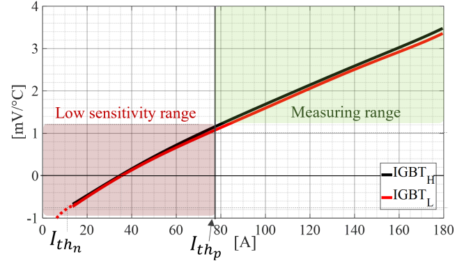
Fig. 11. Average sensitivity curve for phase U high-side and low-side IGBTs.
