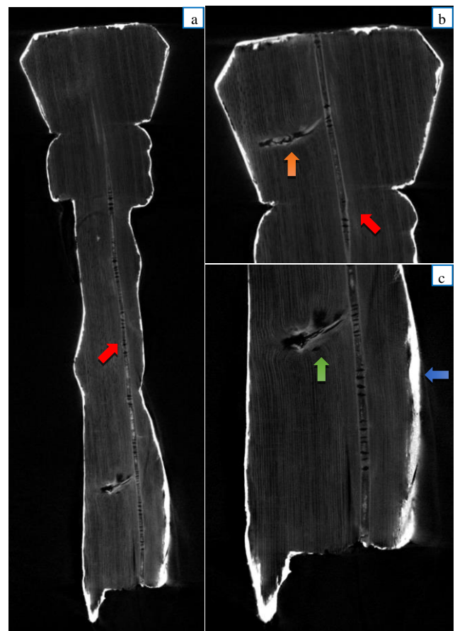
Fig.3. CT vertical slices of statuette B (a: entire figure; b: detail of the basket; c: detail of the body) in which the hole caused from the pith detachment is clearly visible (red arrows: pith; green arrow: knots; blue arrow: thicker preparation layer; orange arrow: crack).
