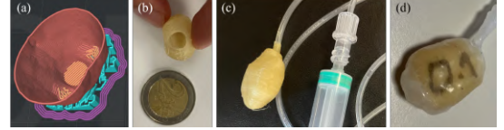
Fig. 5. Stroke phantom manufacturing. (a) 3-D model cut view; (b) PVA mold; (c) Model sealed; (d) Stroke phantom before of remove PVA material.
