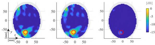
Fig. 8. Transverse views center at the maximum, amplitude normalized of the reconstructed dielectric contrast. (from left to right) Reference scenario 5 \text{ cm}^3 (See Fig. 7(I-d)); Scenario 5 \text{ cm}^3 using a different set of measurements; false-positive scenario, difference between two empty cases normalized at maximum value of I-d. The red circles indicate the contour of the sphere with the volume of 5 \text{ cm}^3 .
