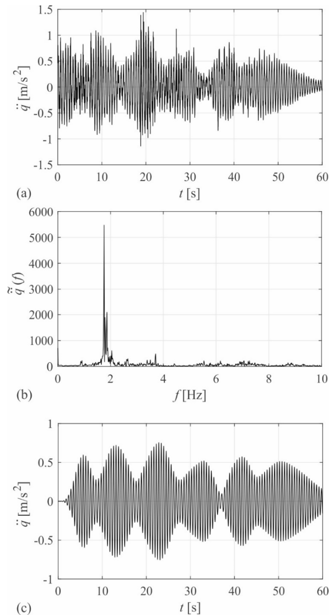
Figure 9. The measured (a) and filtered (c) vertical acceleration and Fourier spectrum (b) by accelerometer 2 (V2) due to a single pedestrian crossing with a step frequency of 1.75 Hz.
