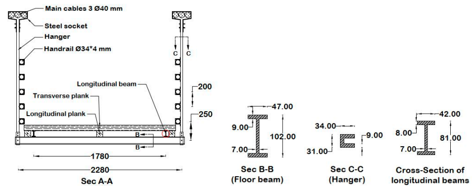
Figure 5. Cross-sections and dimensions of the footbridge structural elements (in mm).
