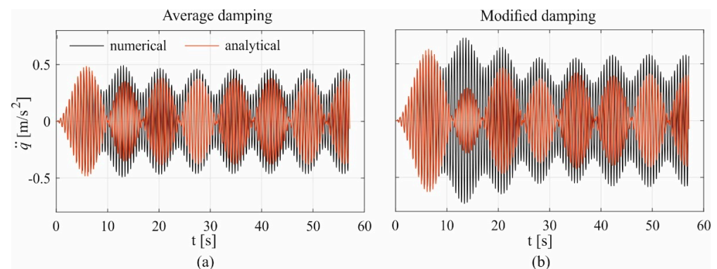
Figure 14. Time history of the acceleration responses by the numerical and analytical solutions predicted with average (a) and modified damping (b) during a single pedestrian crossing with a step frequency of 1.75 Hz.
