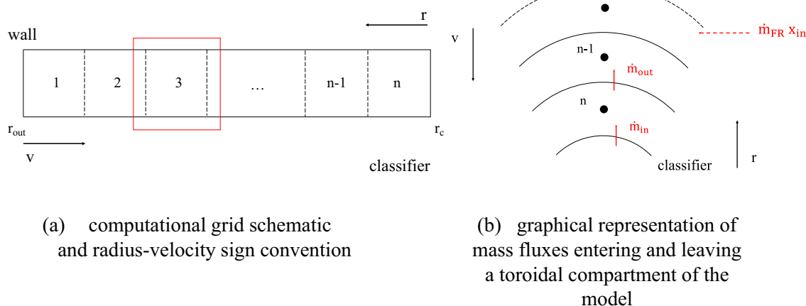
Fig. 9. Spiral jet mill micronization chamber schematization: side view with 1D grid discretization (a) and top view with mass fluxes detail (b).
