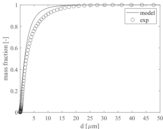
(a) p = 7 \text{ bar(g)} , \text{FR} = 20 \text{ g min}^{-1}
