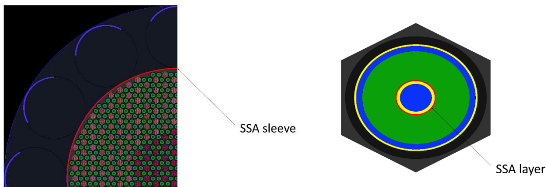
Figure 17 - Reactor configuration with SSA (in red). Left: SSA implemented as a sleeve around the core. Right: SSA implemented as a layer in the moderator elements. SSA thickness not in scale.
