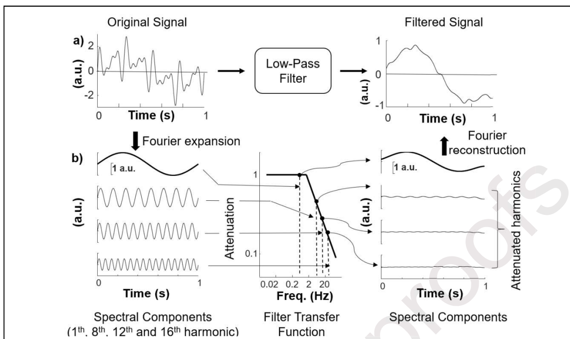
Fig. 10. Operation of a low-pass filter. a) examples of input and output signals of the filter, b) harmonics of the input and output signals of the filter undergoing different attenuations. See text for details.
