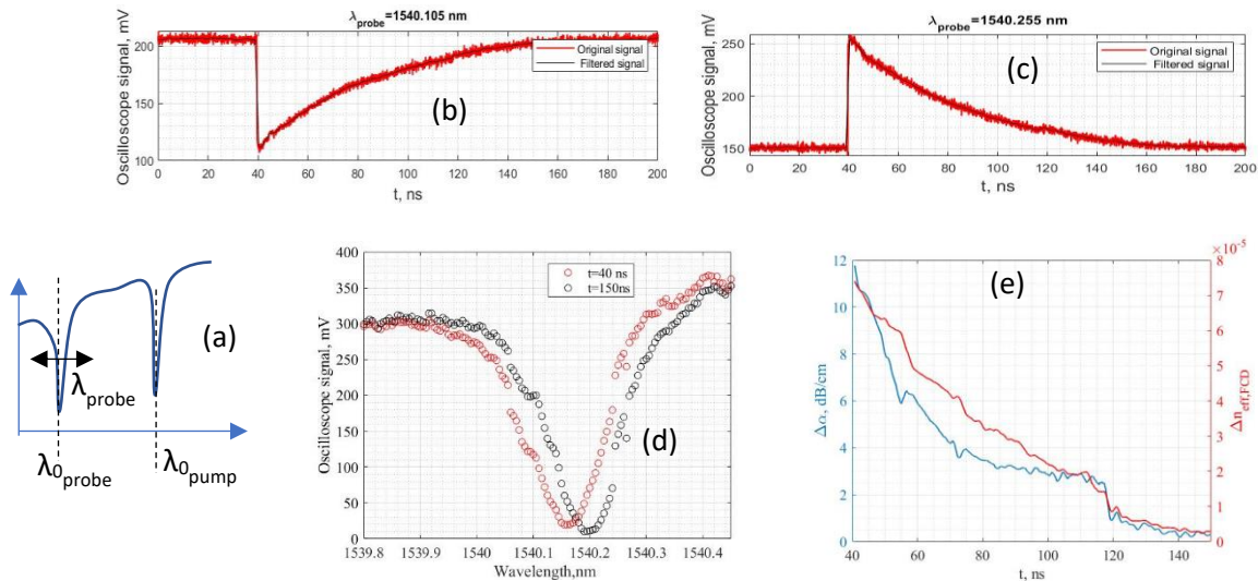
Fig. 4. (a) Schematic of the pump-probe experiment. (b) and (c) show probe powers traces signals recorded at the through port for probe wavelength below (b) and above (c) the cold resonance. (d) Time resolved spectral response of the ring around \lambda_{0,probe} at t = 40 \text{ ns} (just after the pump pulse) and at t = 150 \text{ ns} (when the non-linear transient is concluded and the ring is in linear regime). (e) Extracted variation of effective refractive index due to FCD and non-linear loss in the ring versus time.
