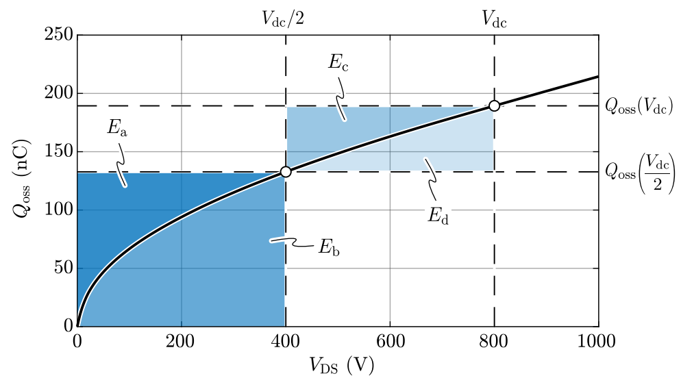
Figure 2. Output charge Q_{\text{oss}} dependence on the drain-source voltage V_{DS} of the Wolfspeed C3M0032120K 1200 V 32 mΩ SiC MOSFET, with highlighted capacitive energy components E_a , E_b , E_c , and E_d , assuming V_{dc} = 800 V.
