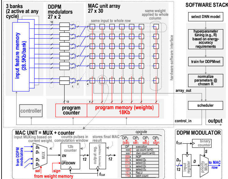
Fig. 3. DDPMnet architecture and underlying software stack.
