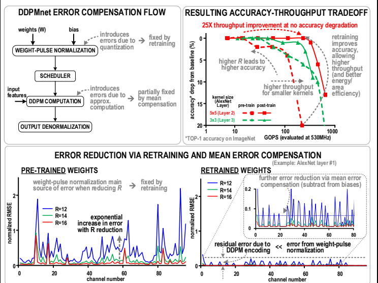
Fig. 4. Error compensation and accuracy recovery using retraining and accuracy-throughput tradeoff.
