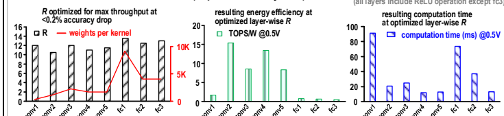
Fig. 5. Performance across datasets, neural networks, and layers along with the benefits of retraining and scheduling.
