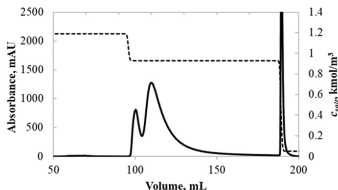
Figure 10. Chromatogram of the reference process (standard process conditions).
