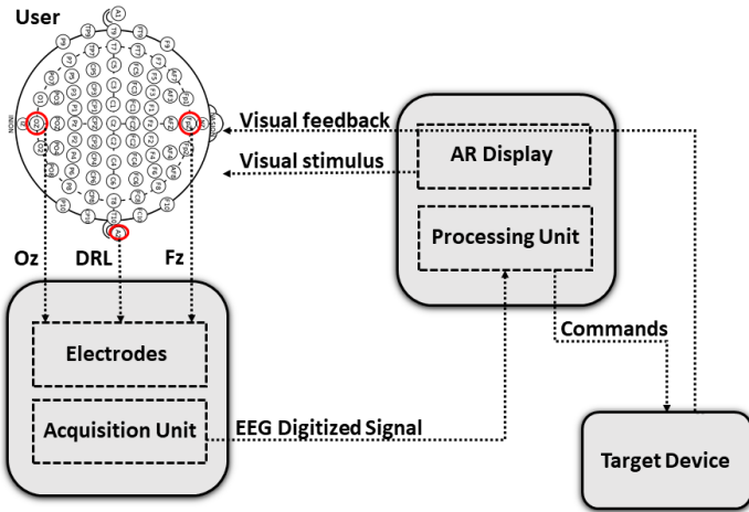
Fig. 1: General architecture of the AR-BCI SSVEP instrumentation.
