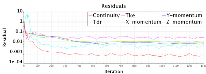
Figure 16 Standard configuration, residuals trend normalized to the value of 0.1
