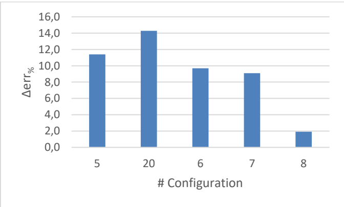
Figure 41 Spoiler's included configuration k- \epsilon
