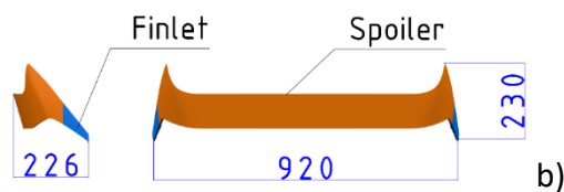
Figure 12 JUNE's Spoiler and Finlet: a) position, b) dimensions
