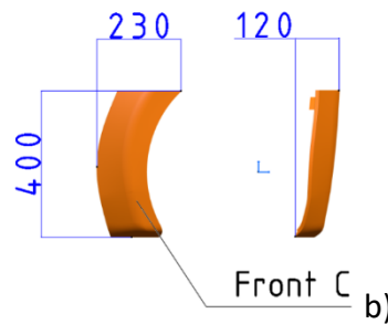
Figure 11 JUNE's Front C: a) position, b) dimensions
