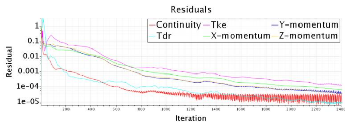
Figure 13 Complete configuration, residuals trend normalized to the value of 0.1
