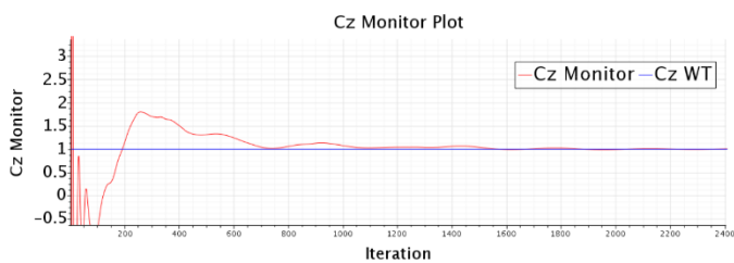
Figure 15 Complete configuration, C_z trend normalized to wind tunnel value
