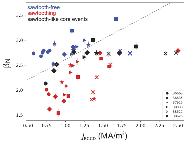
Figure 2. Discharge phases with (red symbols) and without (blue) sawteeth in the parameter space defined by the normalized plasma \beta and the volume-averaged non-inductive central current density. Adapted with permission from [14].
