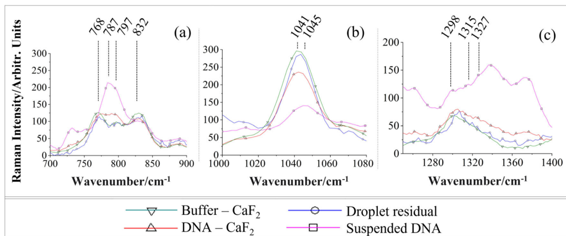
FIGURE 4 Details of the samples with \text{NiCl}_2 + HEPES buffer. Zoomed view of the areas where the spectra of the suspended DNA and of the working buffer solution overlap, more precisely in the ranges (a) 700\text{--}900\text{ cm}^{-1} , (b) 1000\text{--}1080\text{ cm}^{-1} and (c) 1270\text{--}1400\text{ cm}^{-1} . The wavenumber assignment is reported in each panel [Colour figure can be viewed at wileyonlinelibrary.com ]
