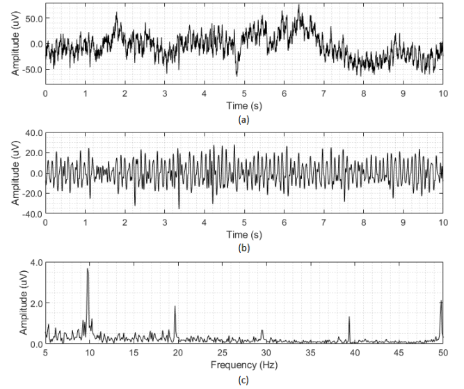
Fig. 1. Example of a SSVEP of a user staring at a 10 Hz-flickering stimulus: EEG in the time domain (a); Filtered EEG in the time domain (b); EEG in the frequency domain (c).
