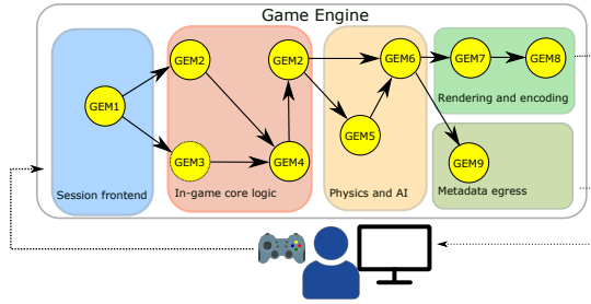
Figure 2: Game session workflow in CODEG.
