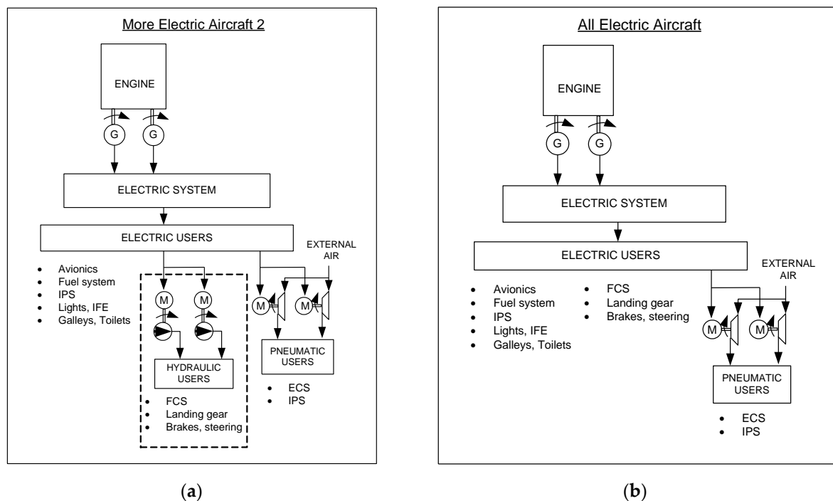
Figure 2. More electric aircraft 2 (a) and all electric (b) OBS architectures.
