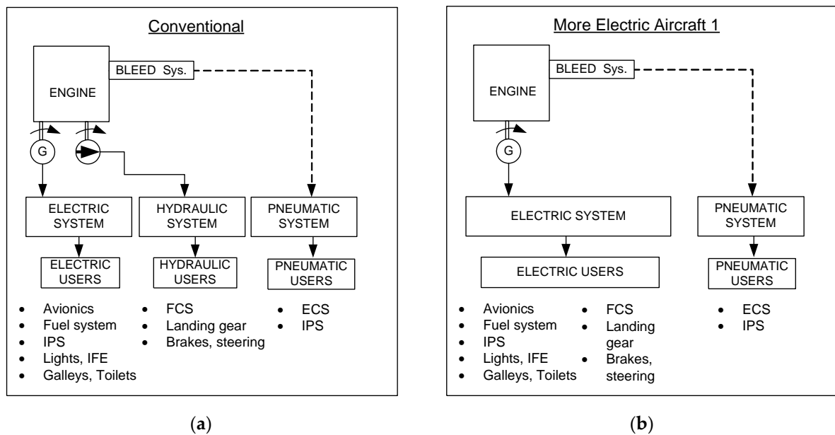
Figure 1. Conventional (a) and more electric aircraft 1 (b) OBS architectures.
